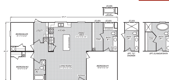
MODEL 28483A 3 Bedroom • 2 Bath • 1,264 Square Feet
