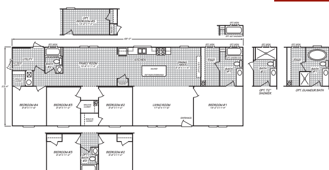
MODEL 24684A 3 Bedroom • 2 Bath • 1,586 Square Feet
