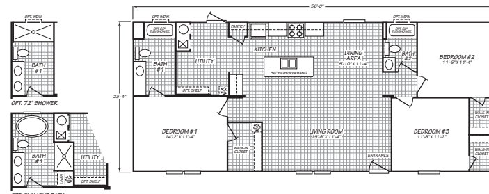
MODEL 24563U 3 Bedroom • 2 Bath • 1,306 Square Feet
